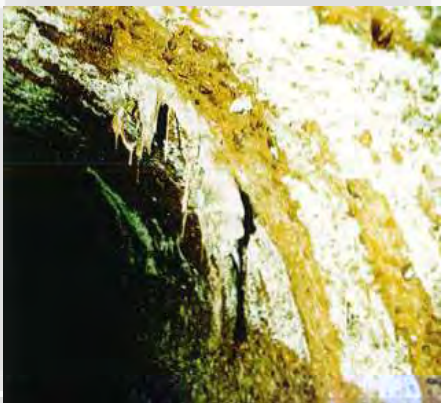
1999 Tunnel Inspection
